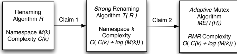
Figure 2: The structure of the reduction in Theorem 1. When C(k) , the complexity of algorithm R , is in o(k) , and M(k) , the target namespace for R , is a sub-exponential function, the RMR complexity of the resulting adaptive mutex algorithm ME(T(R)) is o(k) , contradicting a lower bound by Anderson and Kim [24].
